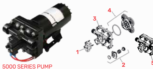
5000 SERIES PUMP
