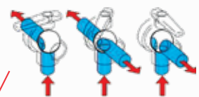
ARAG CONTINUOUS FLOW (H) 3-WAY BALL VALVE
